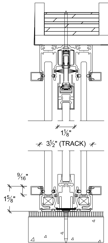
Framed single glazed in open position Verre simple encadré position ouverte
