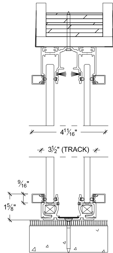
Framed single glazed in closed position Verre simple encadré position fermée
